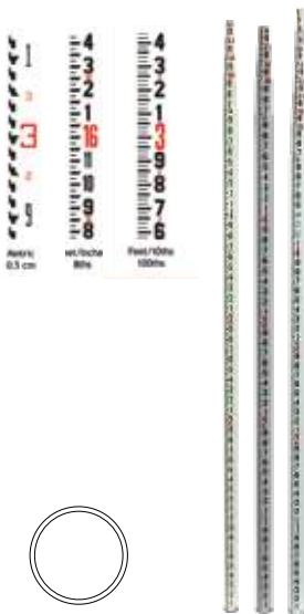
Round design makes the LR Series rods a good choice for certain applications like in areas of high wind.
